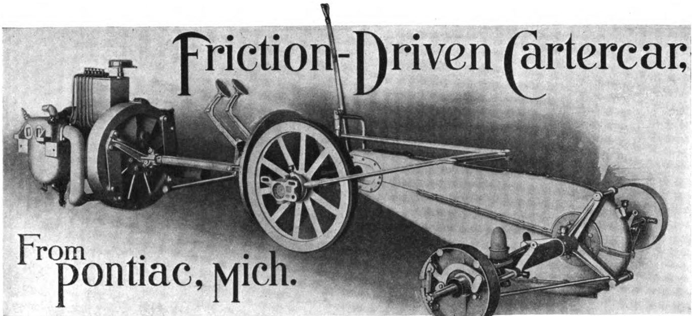
The Friction Drive and Enclosed Chain Make a Very Simple-Looking Outfit.
